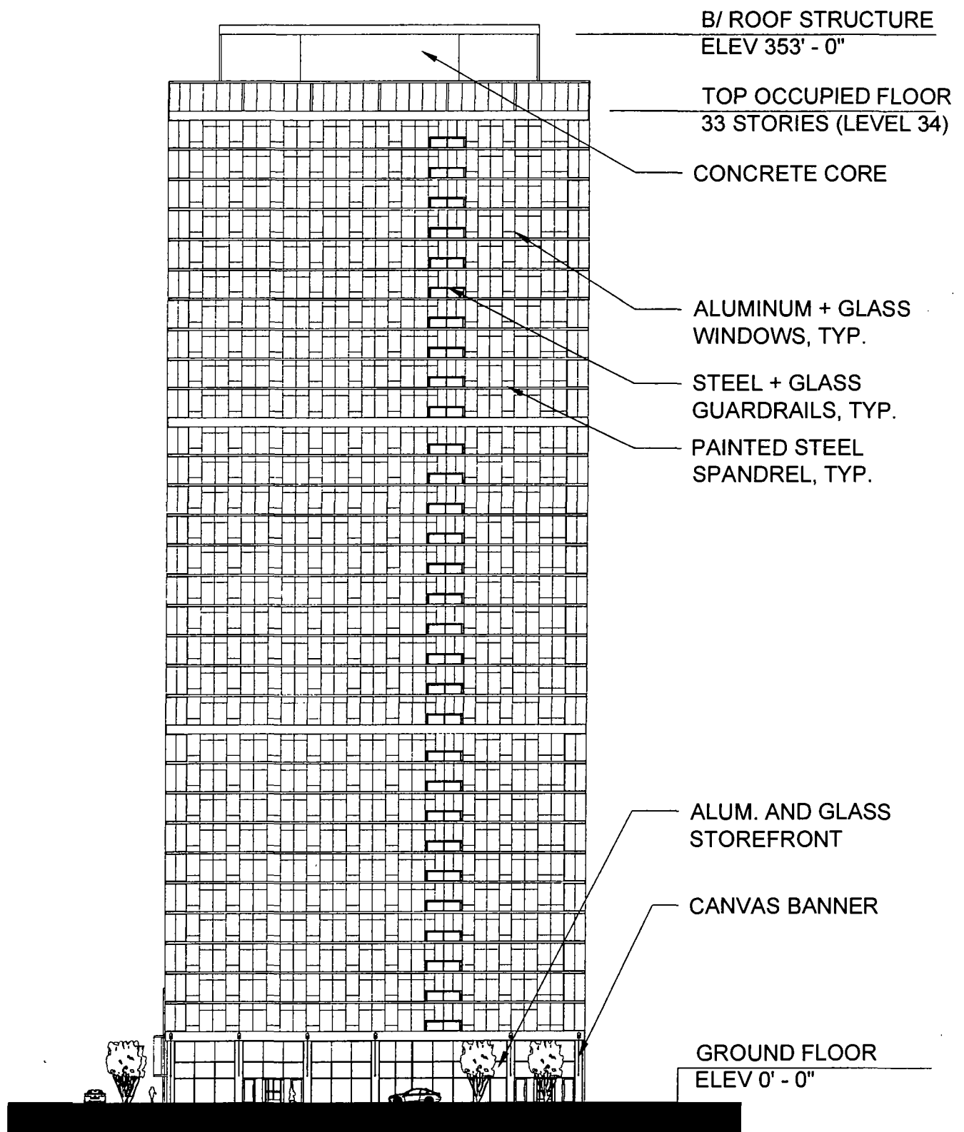
H1. SOUTH ELEVATION ALONG CHICAGO AVENUE
