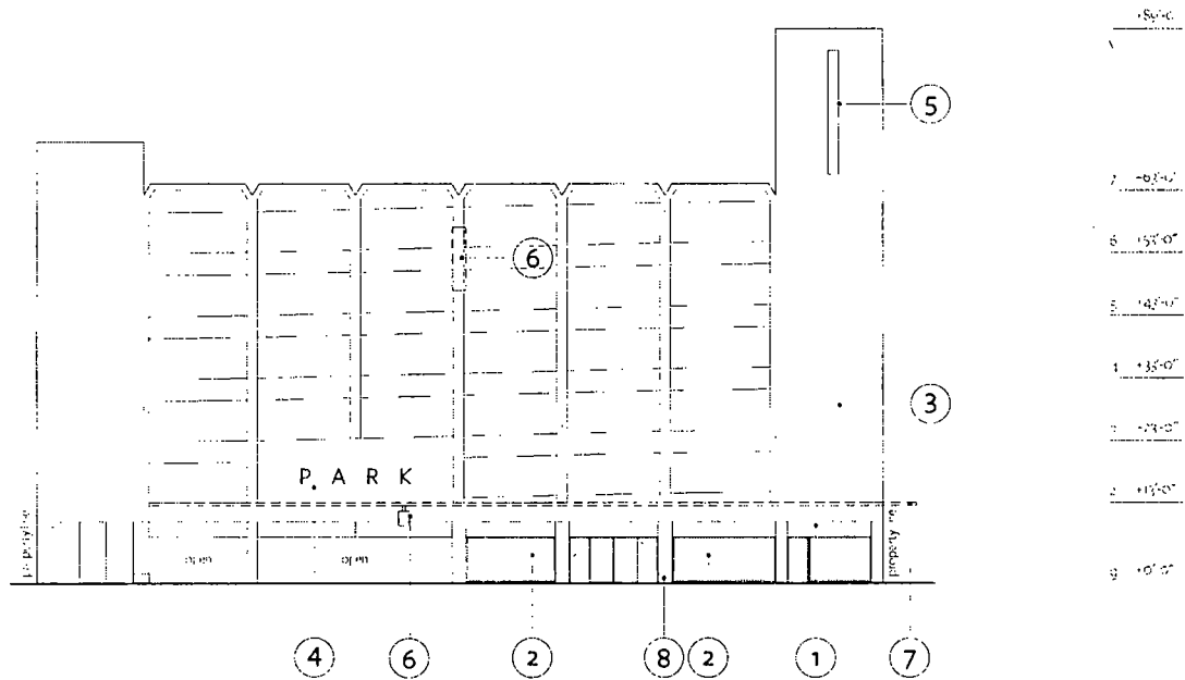
Sub Area B South Elevation Scale: 1/32" = 1'-0"
