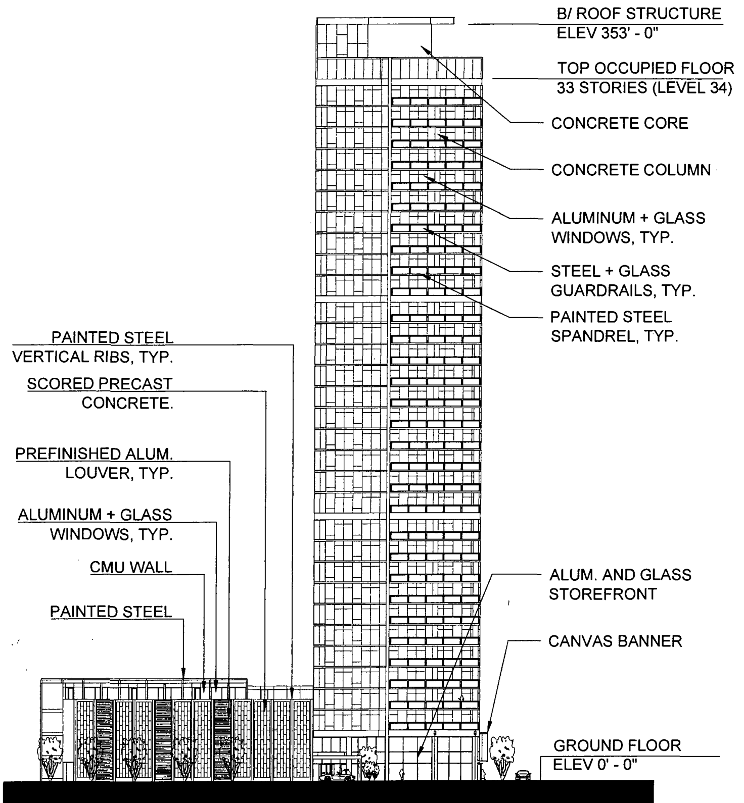
H2. WEST ELEVATION ALONG LASALLE STREET
