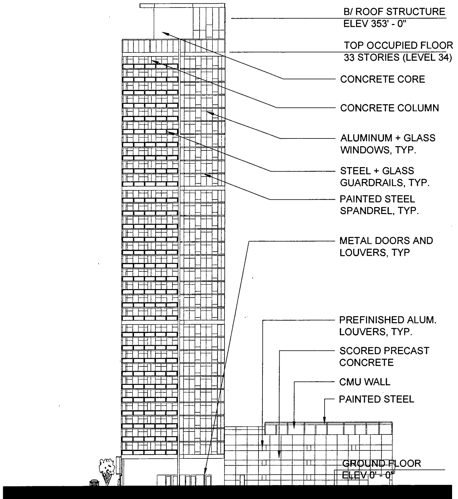
H3. EAST ELEVATION ALONG ALLEY
