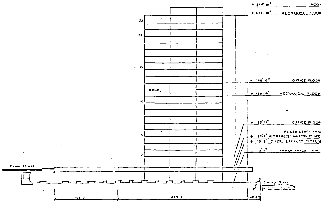
SECTION-LOOKING NORTH
